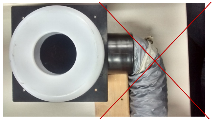
Figure 10: Do not bend the flex duct 90 deg. at the collar
