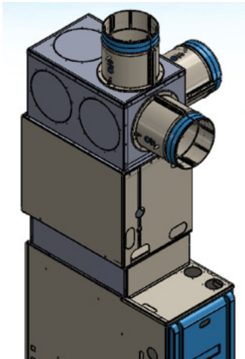
Figure 6: Distribution box
