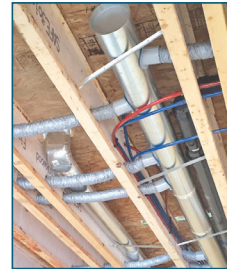
Main trunk and ducts hidden in floor joist
